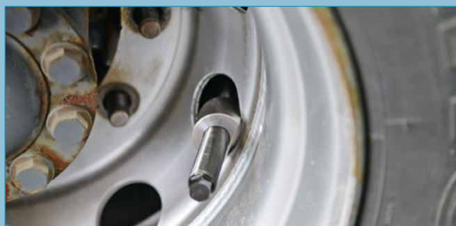
Now operate the spindle until the thrust block (abutment) lies against the inside of the rim hole
