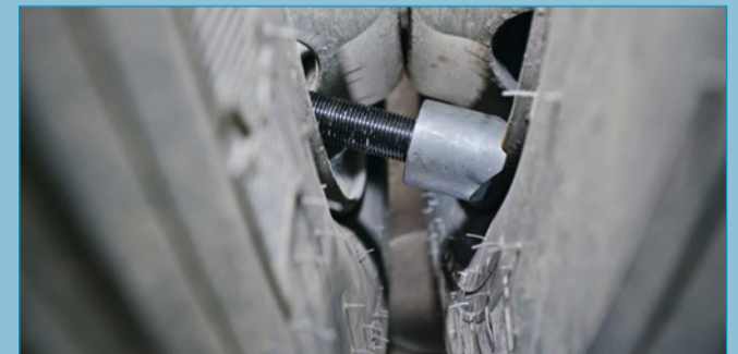
Place the unit in a rim hole. Attention: The rim flange support groove must fit perfectly onto the rim flange of the rear rim
