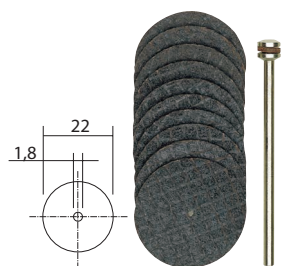
NO 28 808 10 pieces Aluminium oxide cutting discs with reinforcement
